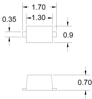
Package Dimensions
