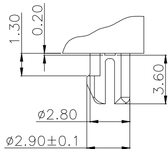
DETAIL "X" SCALE 2:1
