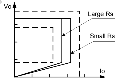
Figure.2 Adjustable output power by changing R_s
