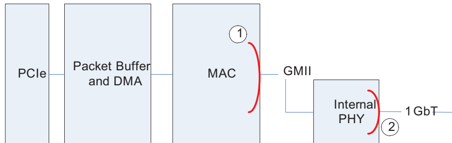
Figure 3-5. I211 Loopback Modes
