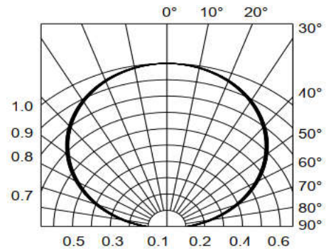
Fig.6-Radiation Diagram Ta=25°C
