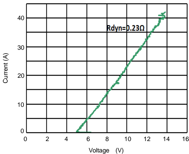
Fig 6. TLP Measurement
