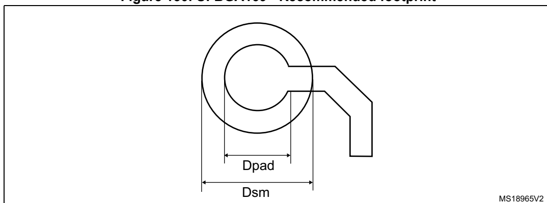
Figure 130. UFBGA169 - Recommended footprint
