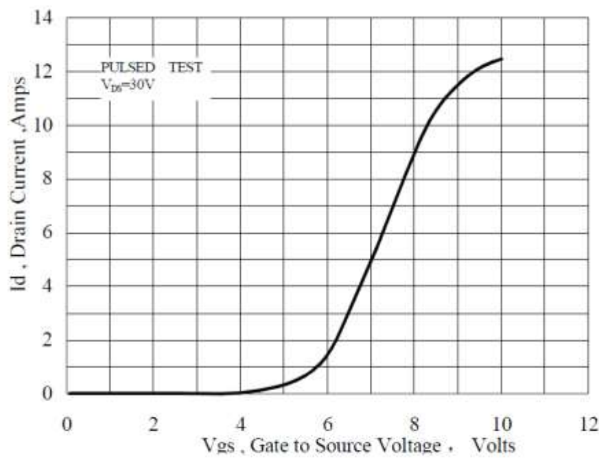
Figure 7 Typical Transfer Characteristics
