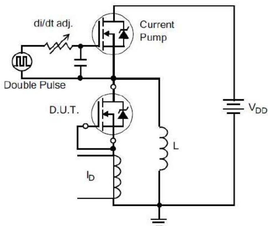
Figure 21. Diode Reverse Recovery Test Circuit
