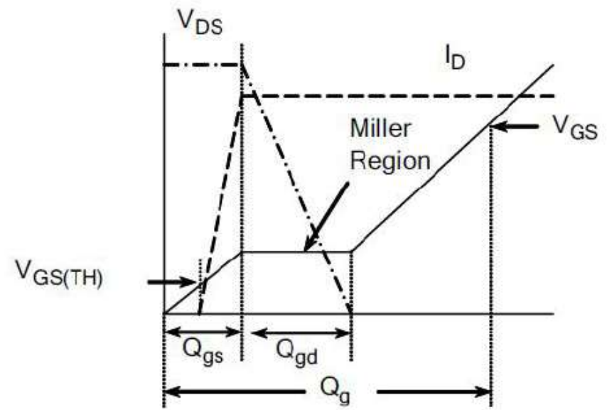
Figure 18. Gate Charge Waveform
