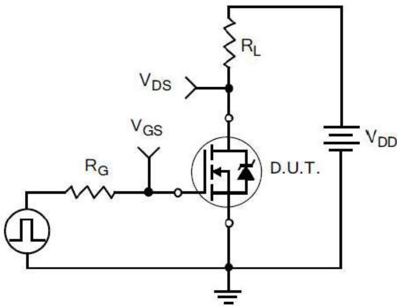
Figure 19. Resistive Switching Test Circuit
