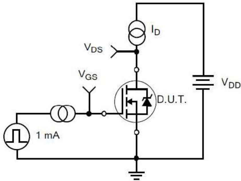
Figure 17. Gate Charge Test Circuit
