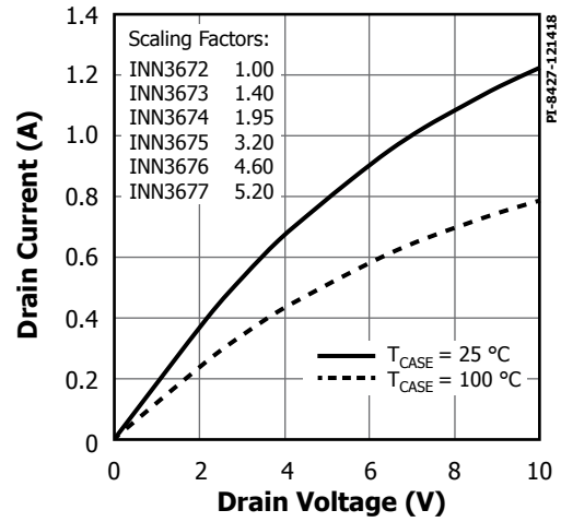
Figure 25. Output Characteristics.
