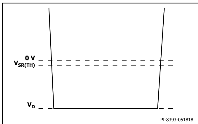
Diode Conduction During Flyback Cycle.
