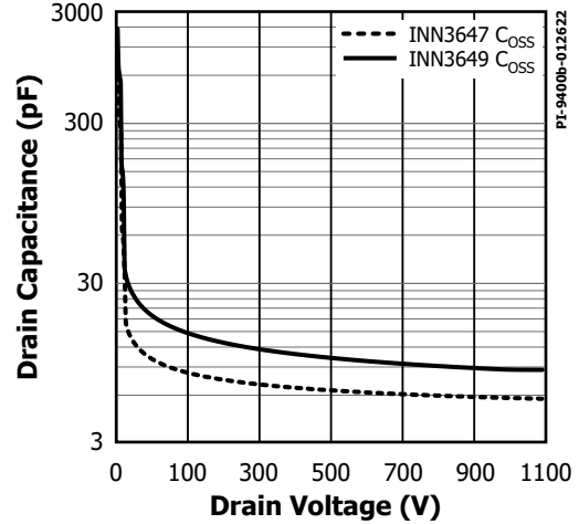
Figure 40. C_{oss} vs. Drain Voltage.
