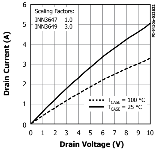
Figure 41. Output Characteristics.
