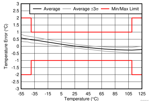
Temperature Accuracy
