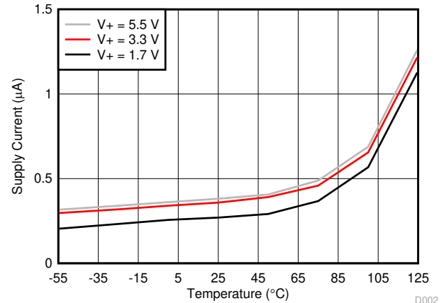
Figure 8-4. Shutdown Current vs. Temperature
