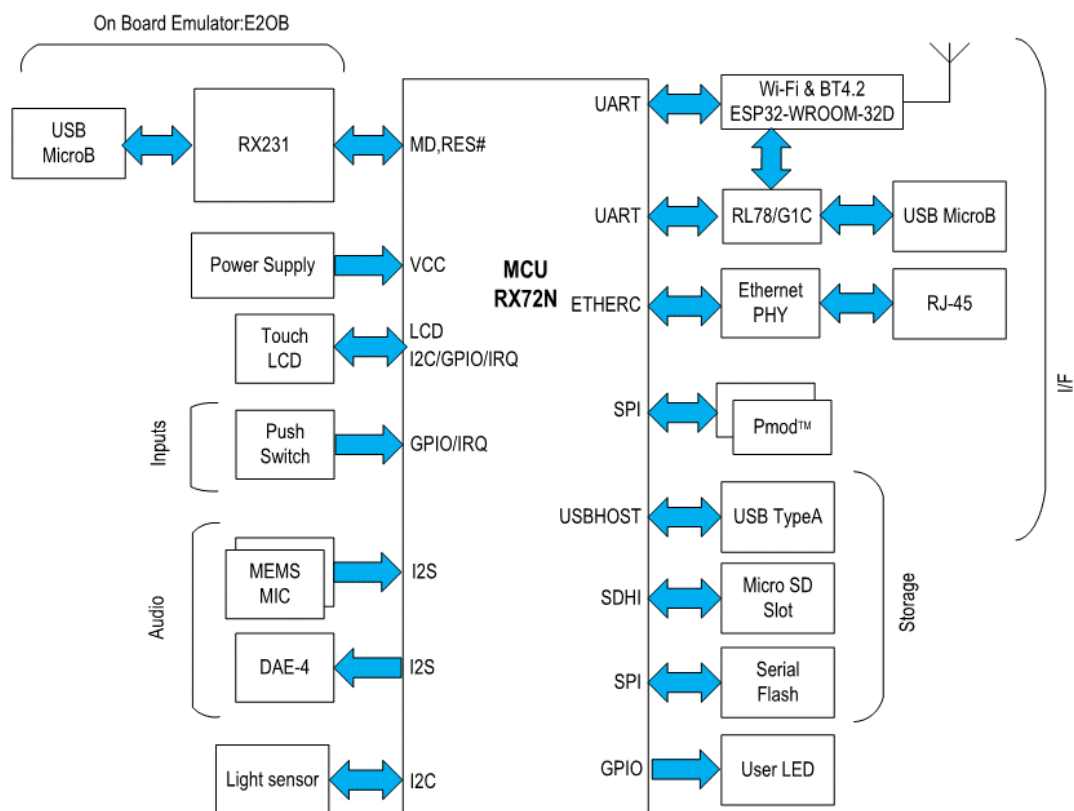
Figure 1-1. Block Diagram
