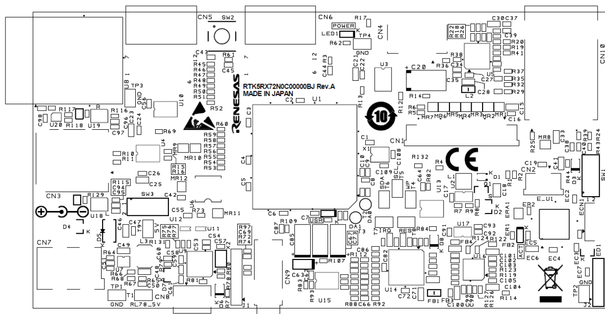
Figure 3-1. Component Layout Diagram
