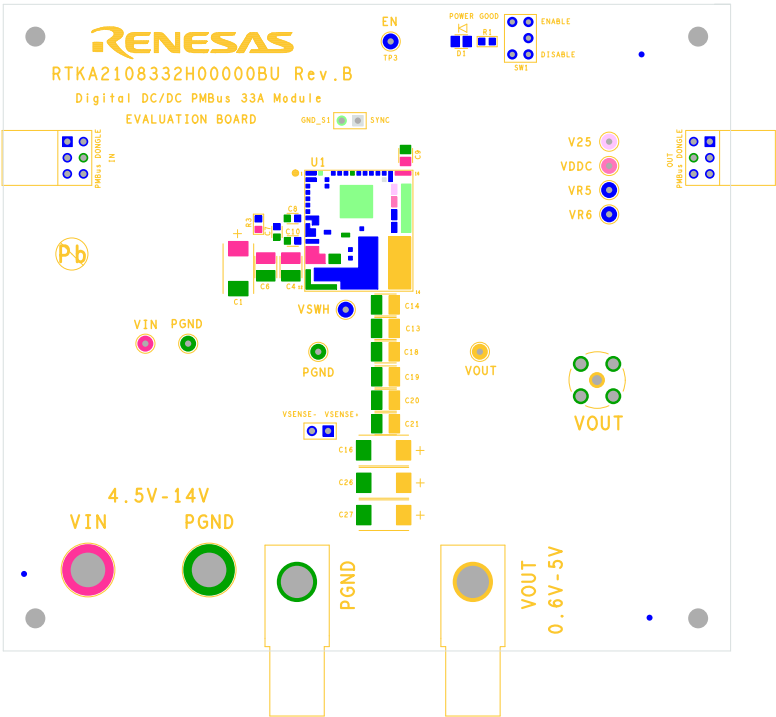
Figure 7. Silkscreen Top
