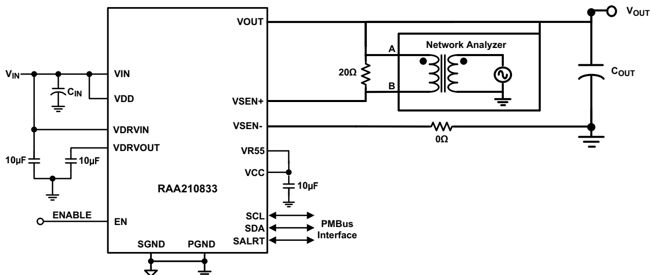
Figure 2. Network Analyzer Connection
