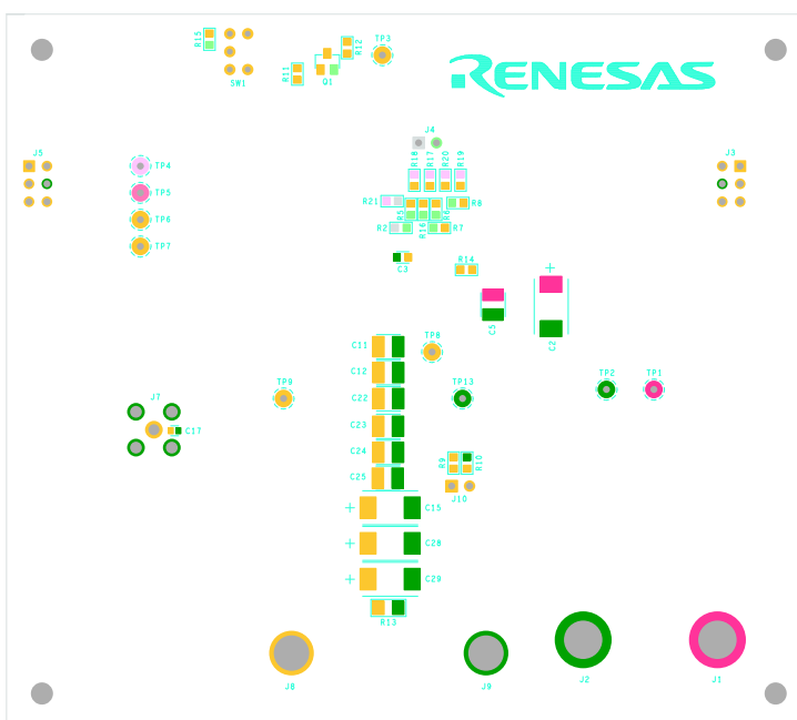
Figure 12. Silkscreen Bottom
