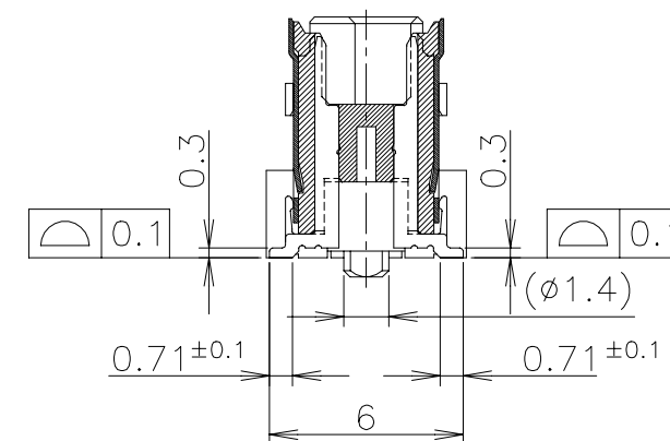
SECT. Z-Z (SIGNAL POSITION)
