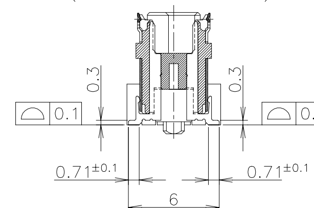
SECT. Y-Y (GROUND POSITION)
