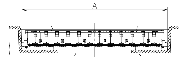
SECT. D-D (SCALE 2:1) (CONNECTOR NOT SECTION)
