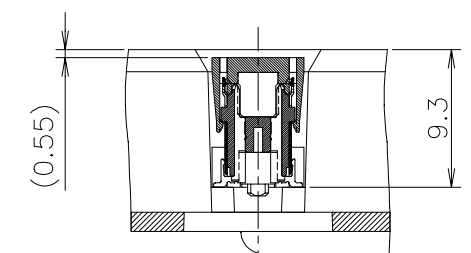
SECT. D-D (SCALE 2:1)
