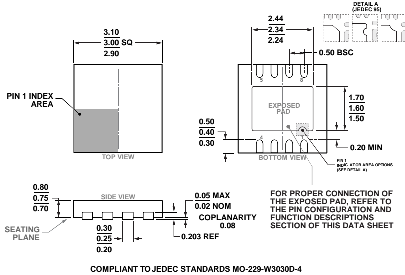
COMPLIANT TO JEDEC STANDARDS MO-229-W3030D-4 Figure 75. 8-Lead Lead Frame Chip Scale Package [LFCSP] 3 mm x 3 mm Body and 0.75 mm Package Height (CP-8-11) Dimensions shown in millimeters
