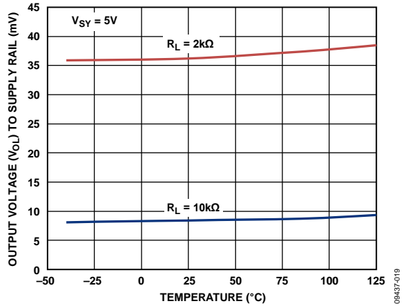
Figure 24. Output Voltage ( V_{OL} ) to Supply Rail vs. Temperature
