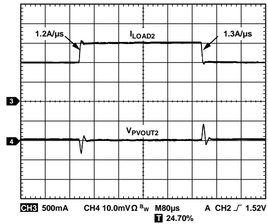
Figure 37. Adaptive Mode Load Transient, V_{PVIN1} = 12\text{ V} , V_{PVOUT2} = 3.3\text{ V} , I_{LOAD2} = 1\text{ A to }1.5\text{ A} , f_{SW} = 1.5\text{ MHz} , L = 2.2\text{ }\mu\text{H} , R_C = 3.48\text{ k}\Omega , C_C = 22\text{ nF} , C_{CP} = 22\text{ pF} , C_{PVOUT1} = 64\text{ }\mu\text{F}
