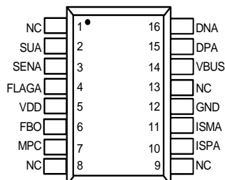
P5 Package CPC-16L
