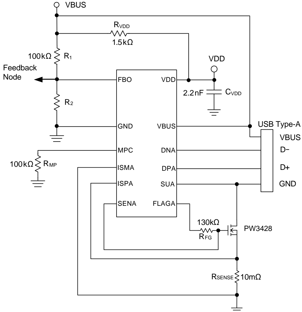
Figure 2. FP6601AM Single Port Typical Application Schematic
