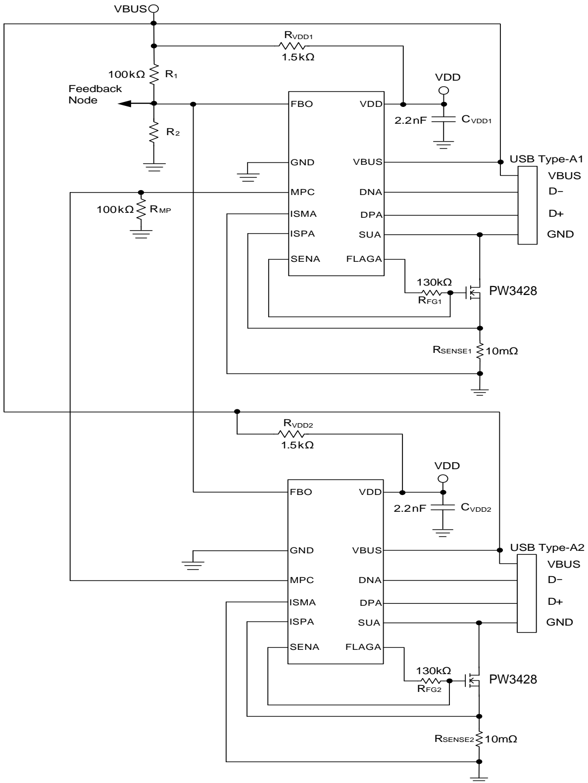
Figure 3. FP6601AM Multi-Ports Typical Application Schematic
