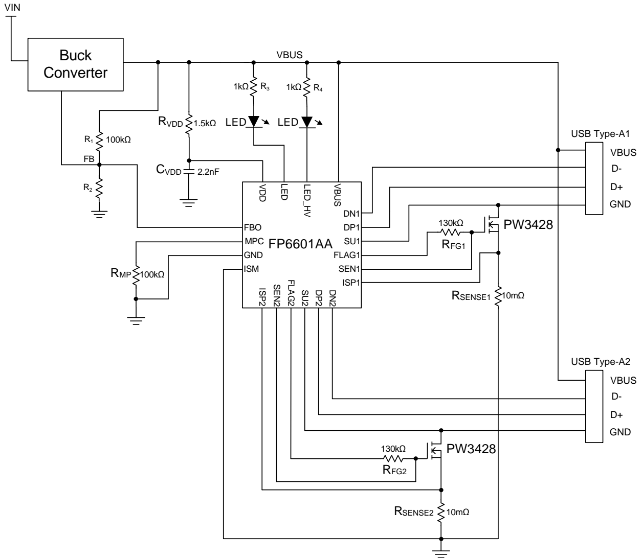
Figure 1. FP6601AA Typical Application Schematic
