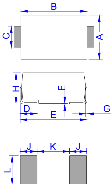
DO-214AA (SMB)
