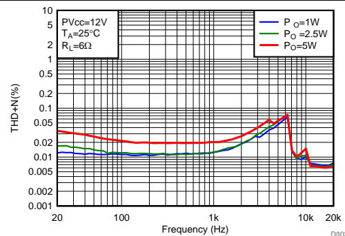
PVDD = 12 V 4.7uH+0.68uF F SW = 768 kHz 1SPW Modulation Load = 6Ω
