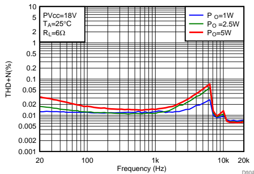
PVDD = 18 V 10uH+0.68uF F SW = 768 kHz 1SPW Modulation Load = 6Ω
