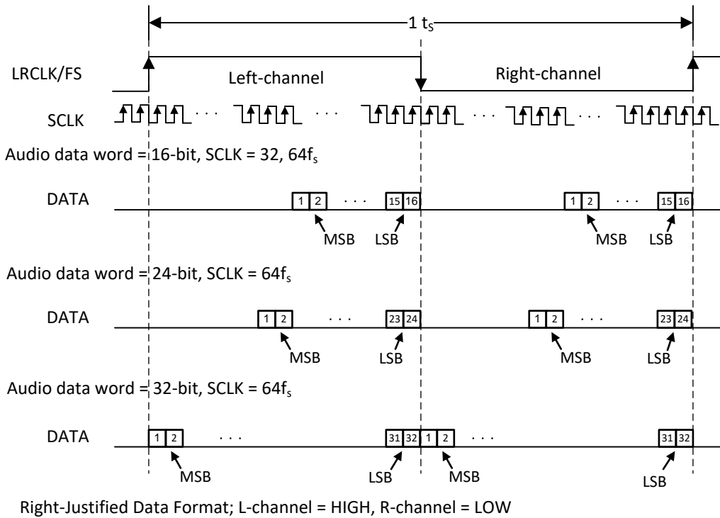
Figure 87. Right-Justified Audio Data Format
