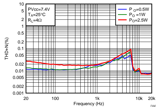
PVDD = 7.4 V 4.7uH+0.68uF F SW = 576 kHz 1SPW Modulation Load = 4Ω
