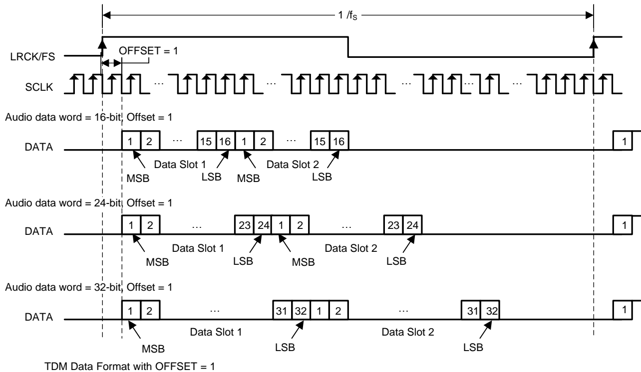
Figure 89. TDM 2 Audio Data Format
