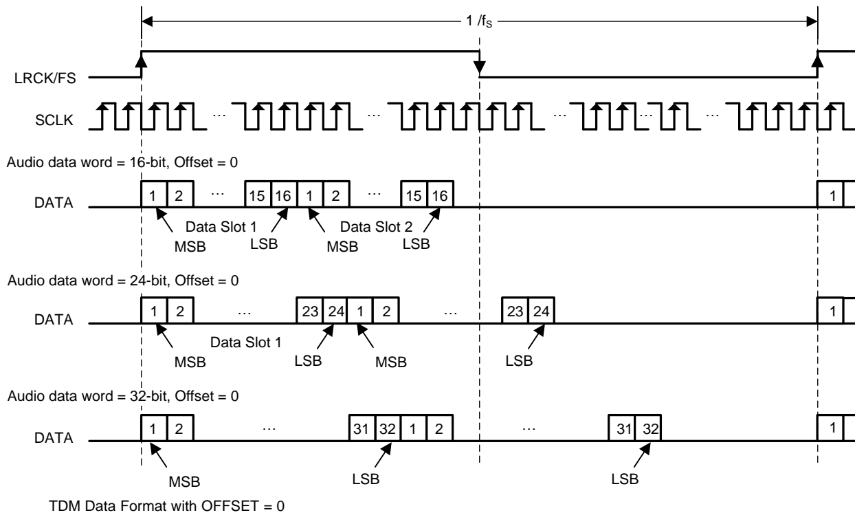
Figure 88. TDM 1 Audio Data Format
