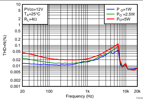
PVDD = 12 V 4.7uH+0.68uF F SW = 768 kHz 1SPW Modulation Load = 4Ω
