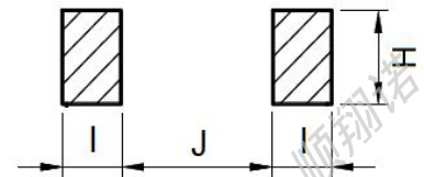
Recommended Land Pattern
