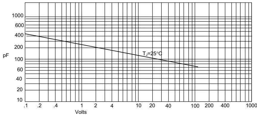
Figure 3 Junction Capacitance
