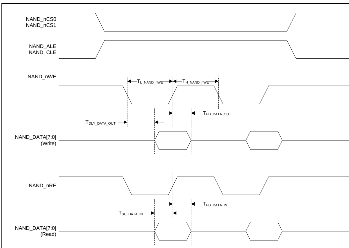
Figure 7.3-11 NAND Interface Timing Diagram
