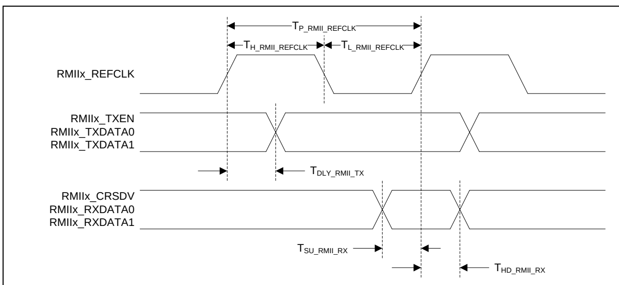
Figure 7.3-9 RMII Interface Timing Diagram
