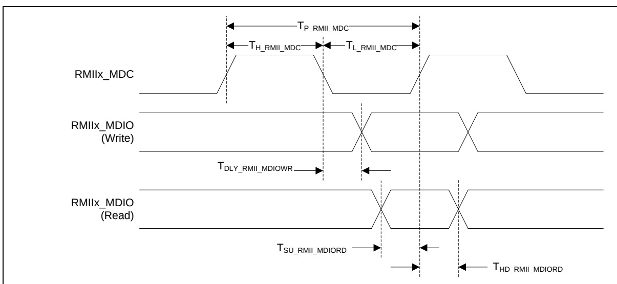
Figure 7.3-10 Ethernet PHY Management Interface Timing Diagram
