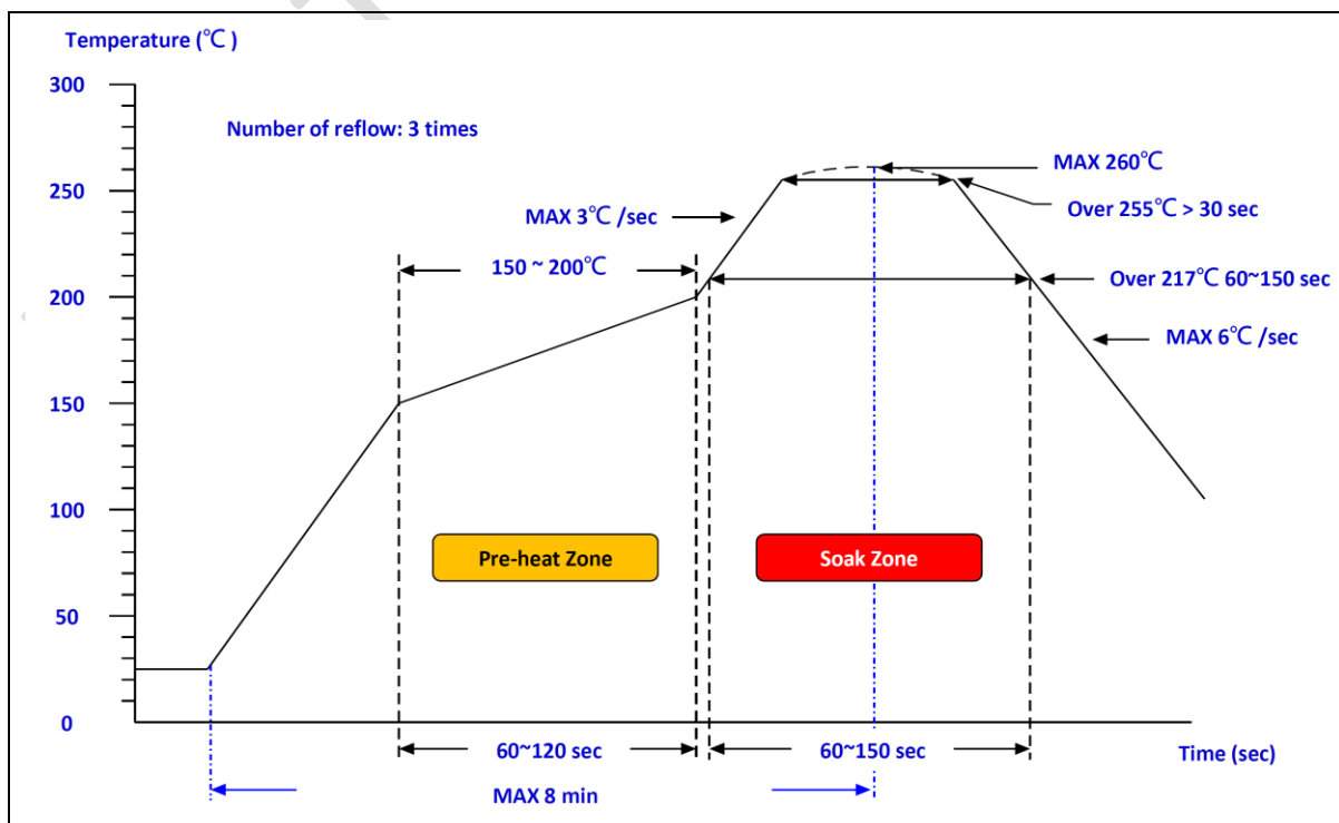
Figure 8.3-1 Profile Suggestion for N9H30 series
