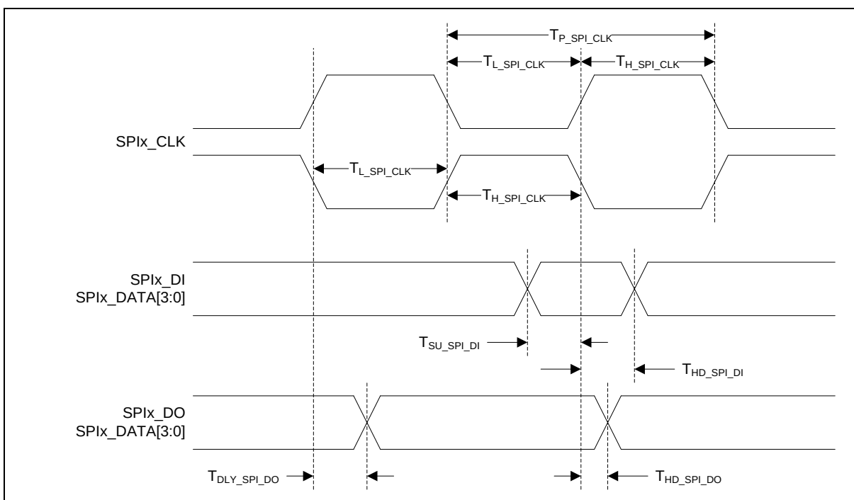
Figure 7.3-7 SPI Interface Timing Diagram
