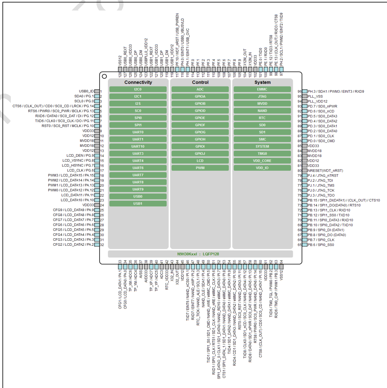
Figure 3.3-1 N9H30KxxI Series LQFP 128-pin Pin Diagram
