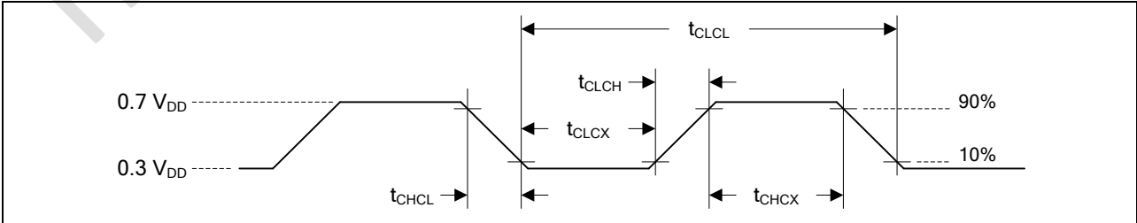
Figure 7.3-1 External 12 MHz High Speed Oscillator Timing Diagram
