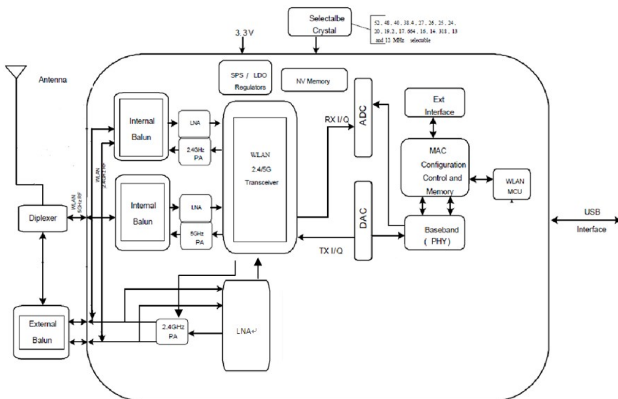
Figure 3 BL-M8811CU2 block diagram
