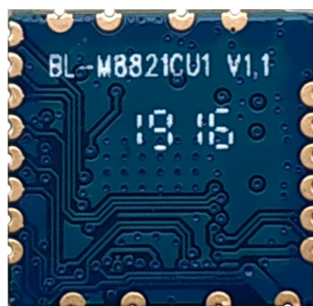
Figure 2 Bottom View
