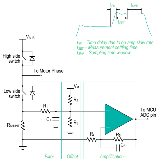
Figure 8. Current Shunt Monitor Circuit
