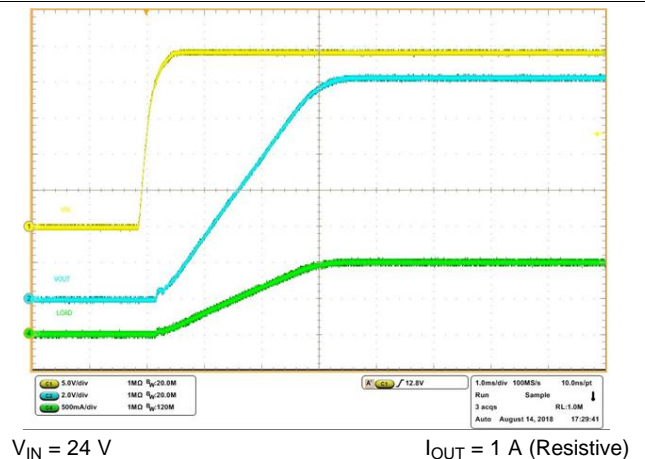
图 18. Full-Load Start-up with VIN
