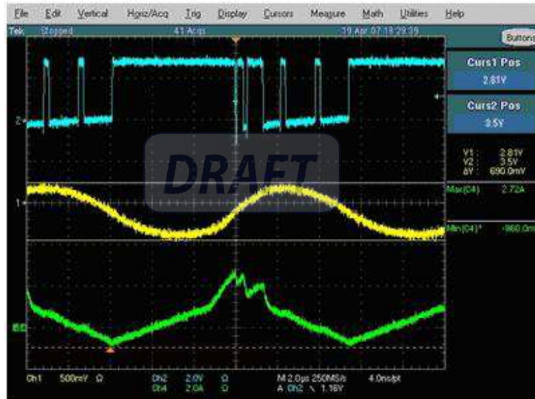
Figure 19. Ceramic 10μF (Y5V) (Bad)
