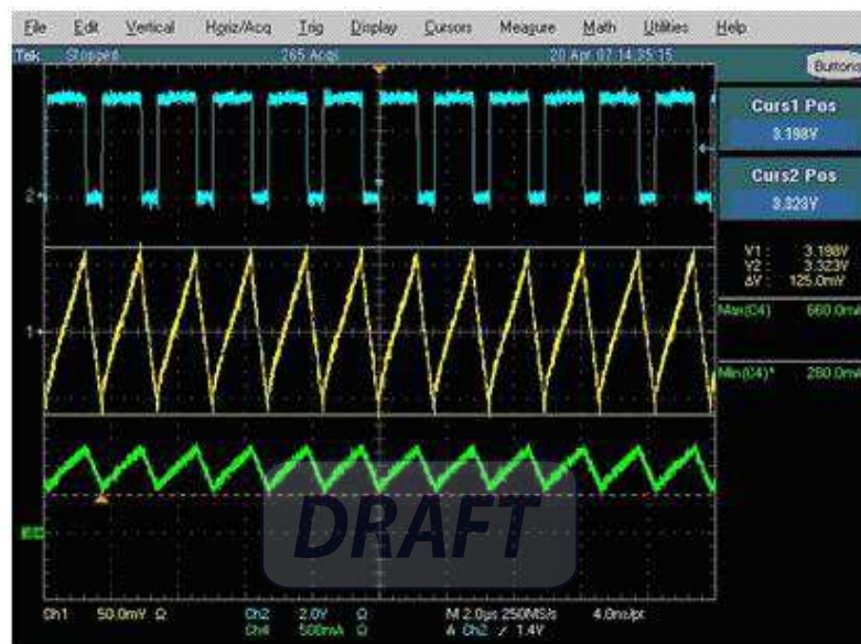
Figure 20. Electrolytic 100μF (Ripple Too High)
