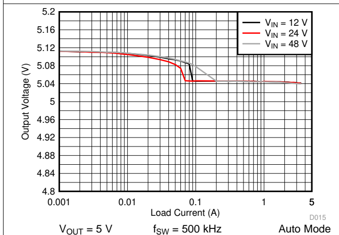
图 39. LM76003 Load and Line Regulation
