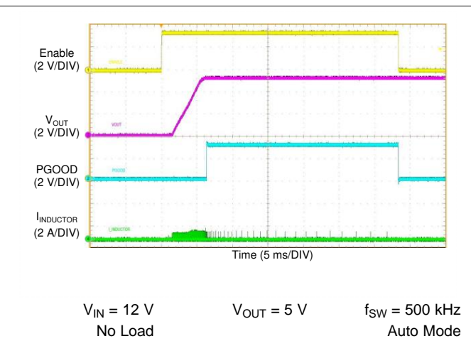
图 64. LM76003 Start-up Waveform
