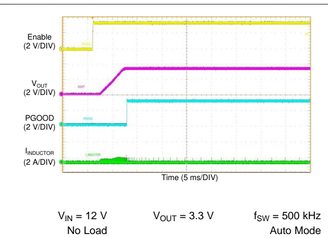
图 62. LM76003 Start-up Waveform
