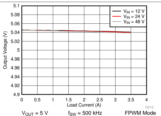
图 40. LM76003 Load and Line Regulation
