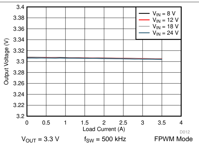
图 38. LM76003 Load and Line Regulation
