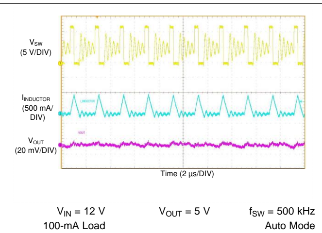
图 60. LM76003 Switching Waveform and Output Ripple
