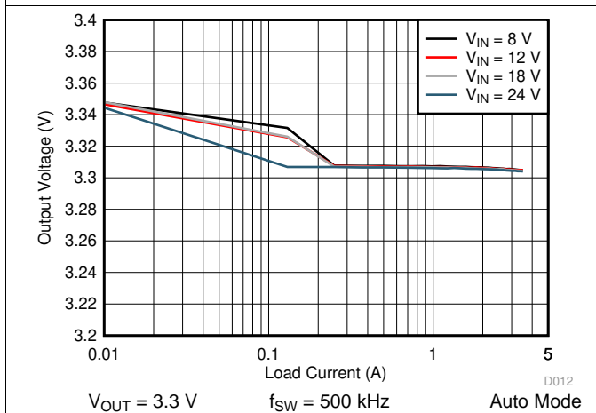
图 37. LM76003 Load and Line Regulation
