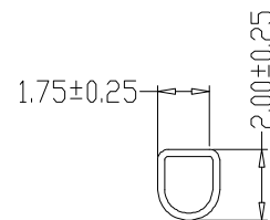
SEC:C-C
