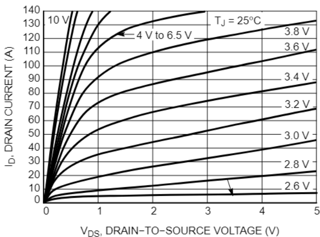
Figure 16. On-Region Characteristics
