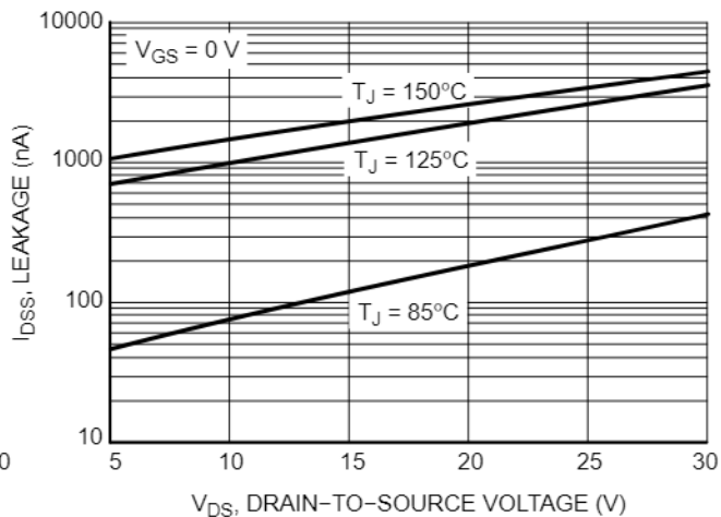
Figure 21. Drain-to-Source Leakage Current vs. Voltage
