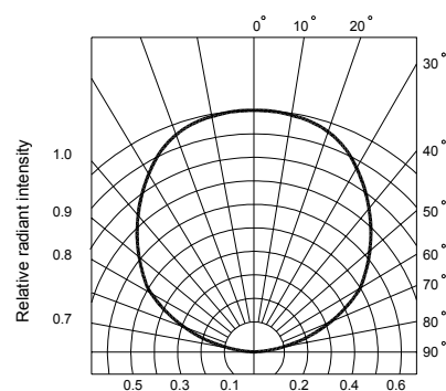
Fig.6 Radiation diagram
