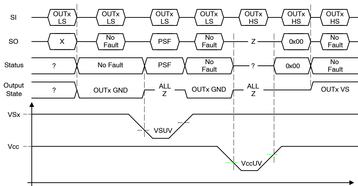
Figure 19. Undervoltage Timing
