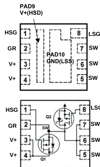
PQFN8 POWER CLIP CASE 483AR
