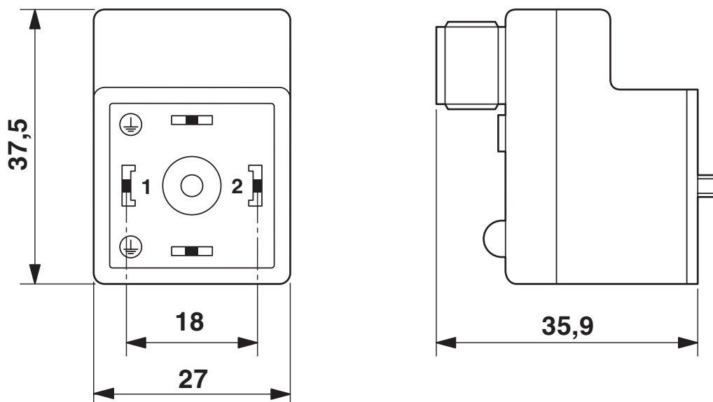
Valve connector, type A with vertical M12 plug
