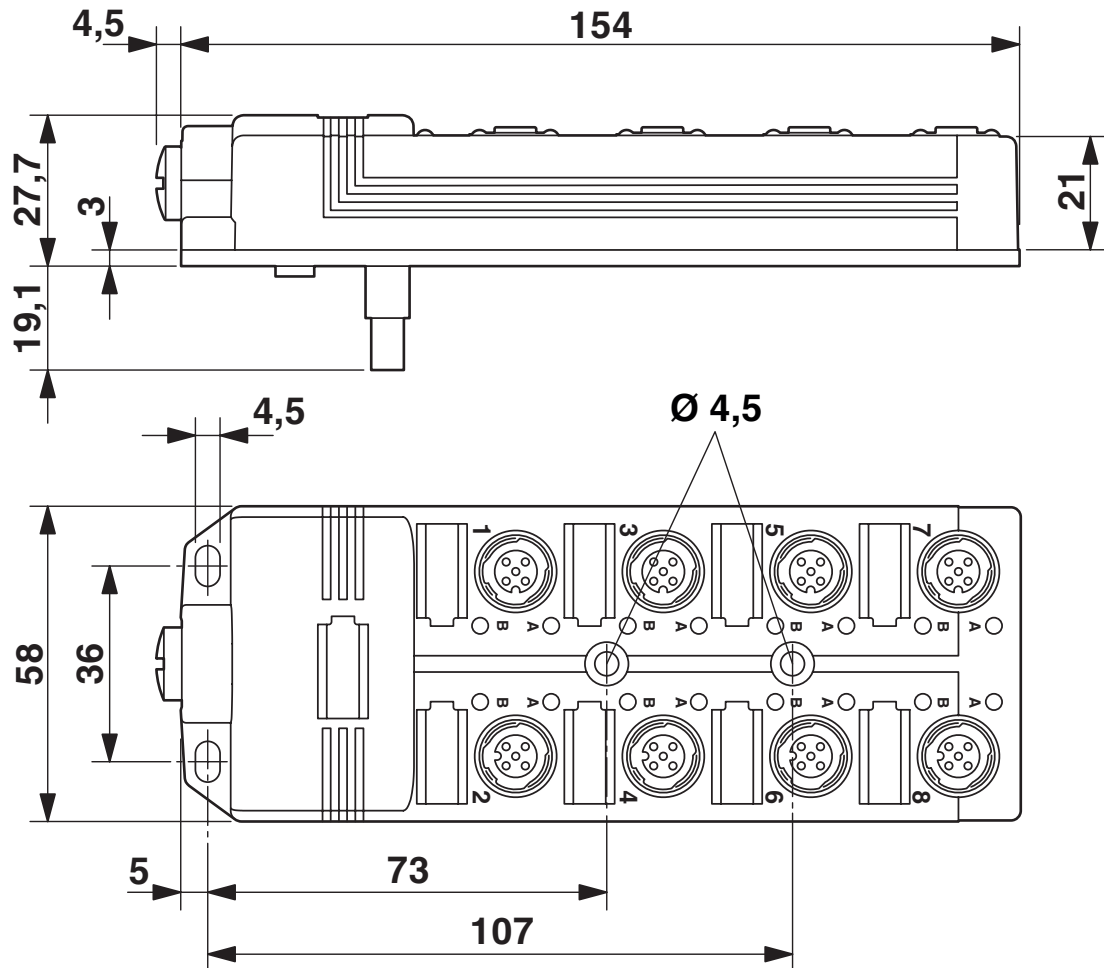
Dimensional drawing
