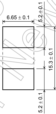
1.2-mm thick metal board
