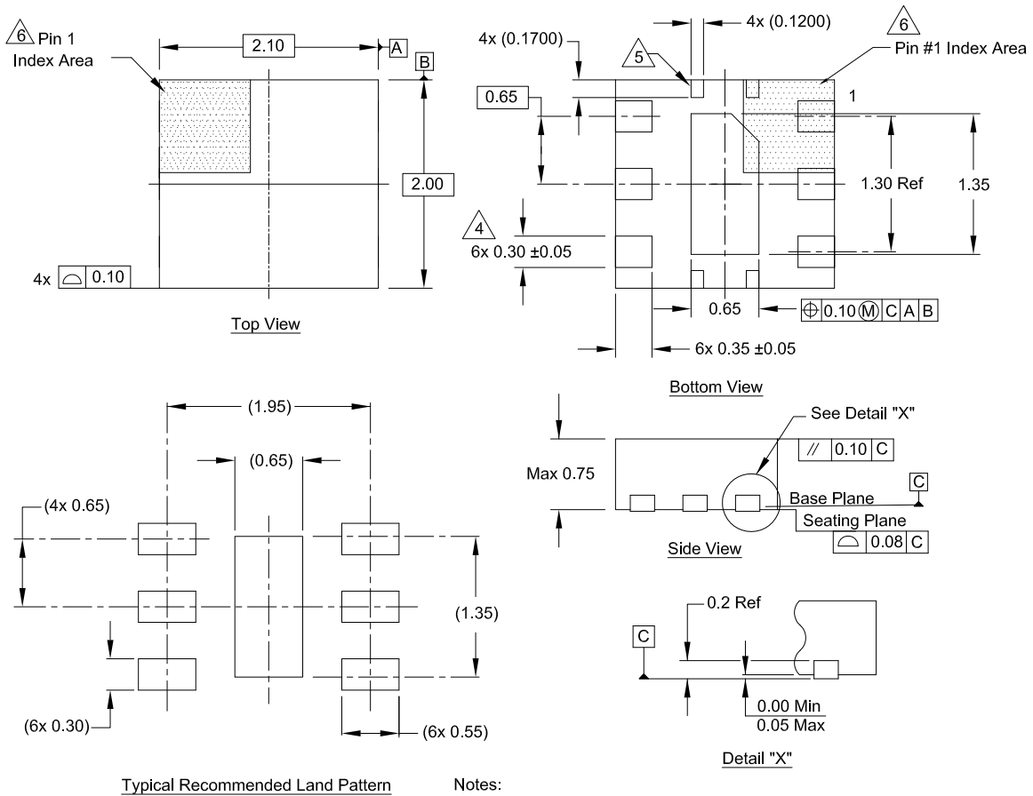
Typical Recommended Land Pattern
