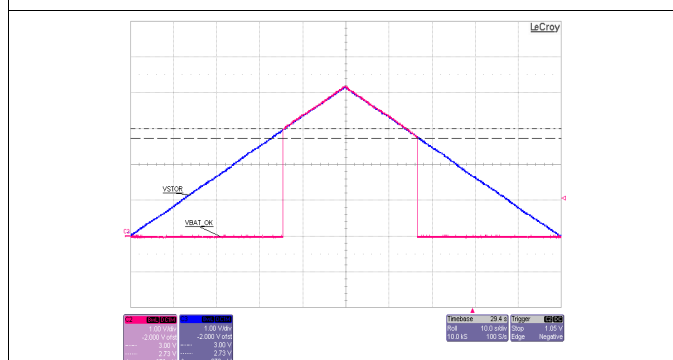
VIN\_DC = 1.5\text{ V} with 75\ \Omega series resistance No storage element on VBAT\_SEC or VBAT\_PRI VSTOR artificially ramped from 0\text{ V} to 4.2\text{ V} to 0\text{ V} using a power amp driven by a function generator
