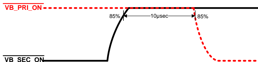
Figure 13. Break-Before-Make Operation of \overline{\text{VB\_PRI\_ON}} and \overline{\text{VB\_SEC\_ON}}
