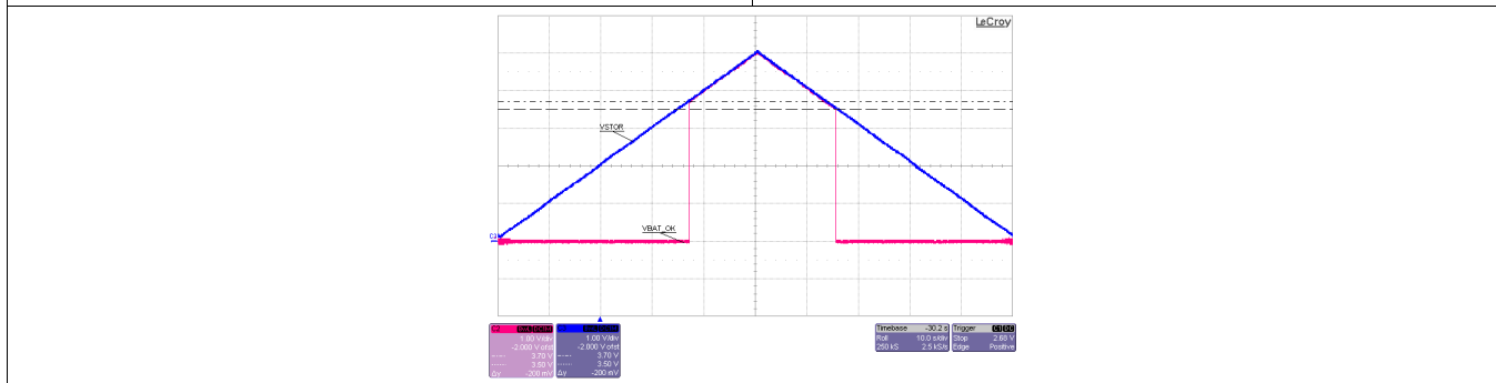
VIN_DC floating No storage element on VBAT or VBAT_PRI VSTOR artificially ramped from 0 V to 5 V to 0 V using a function generator
