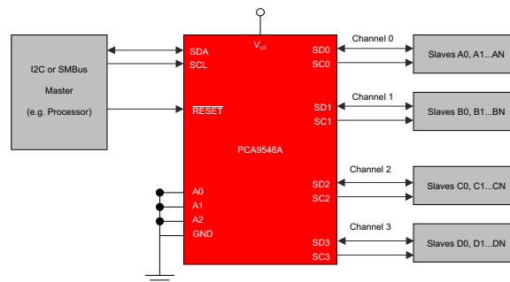
Simplified Application Diagram
