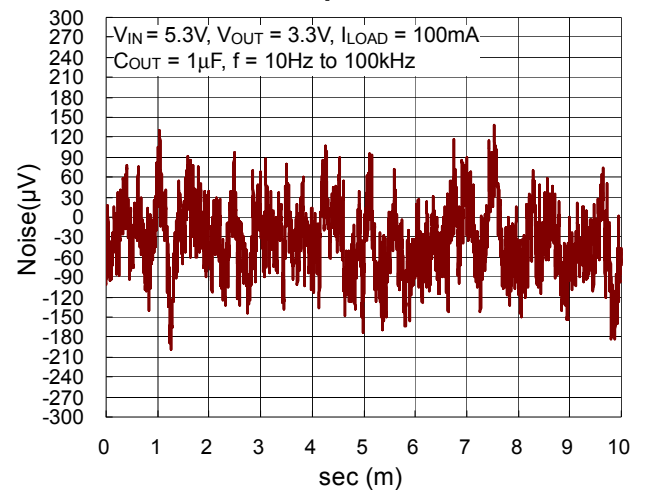
Output Noise
