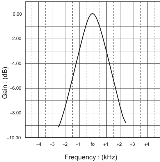
Fig.7 BPF characteristic
