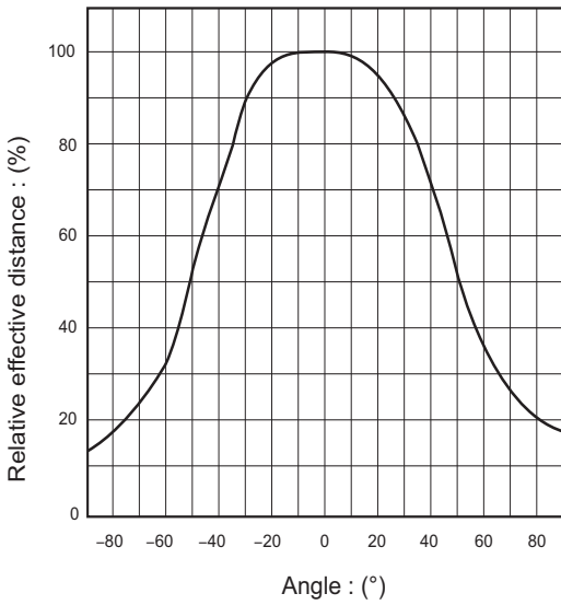
Fig.9 Direction characteristic (Horizontal direction)
