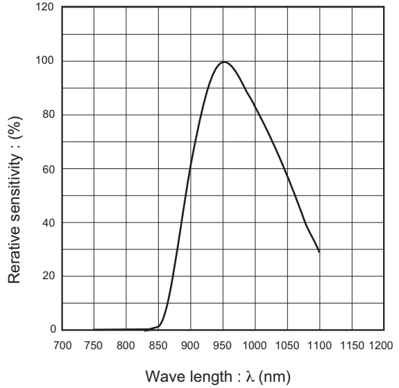
Fig.8 Optical bandwidth of the photo-diode encapsulation
