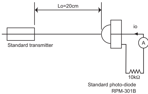
Fig.2 Measurement of standard transmitter proofreading
