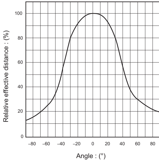
Fig.10 Direction characteristic (Vertical direction)
