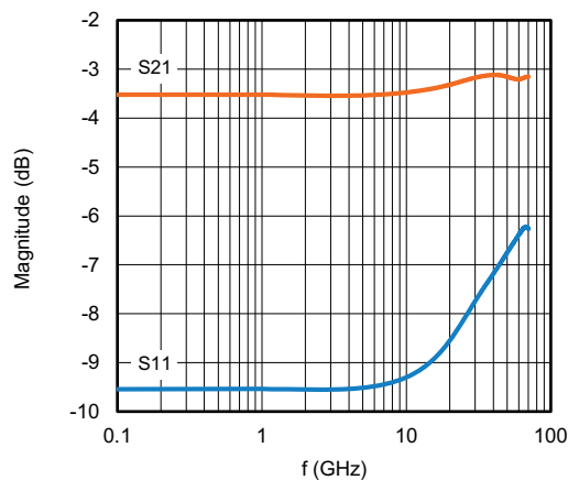
CH02016 flip chip ( Z_0 = Z_1 = Z_s = R = 100 \Omega )
