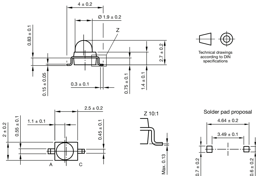
Drawing-No.: 6.544-5325.03-4 Issue: 1; 15.09.2021
