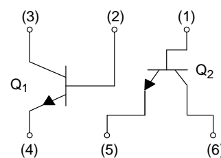
MBT3904DW2T1 STYLE 27
