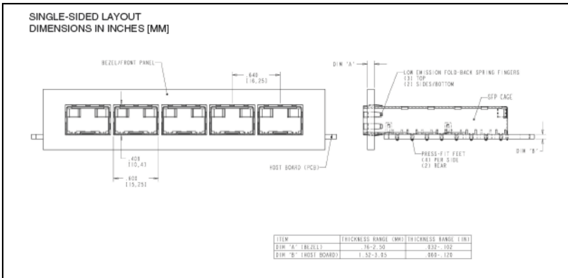
Figure 2 Single-sided Layout
