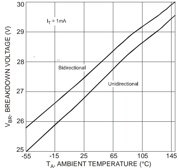
Figure 4 Typical Breakdown Voltage vs. Temperature (MMBZ27VCL)
