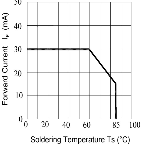
Fig.5-Max.Driving Forward Current vs.Soldering Temperture
