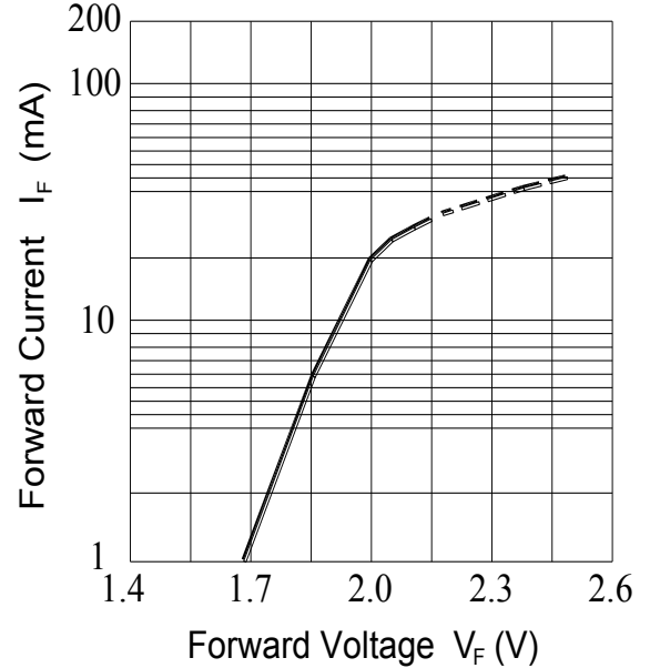
Fig.4-Forward Current vs. Forward Voltage T_a=25^\circ\text{C}
