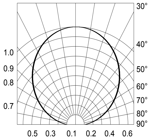
Fig.6-Radiation Diagram T_a=25^\circ\text{C}
