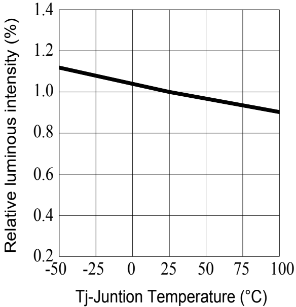
Fig.3-Relative Luminous Intensity vs.Juntion Temperature
