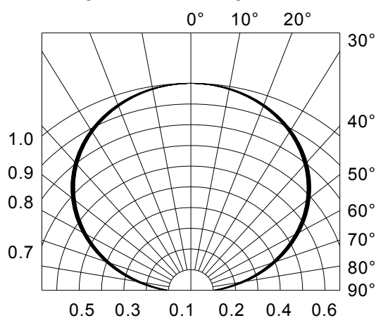
Fig.6-Radiation Diagram Ta=25°C
