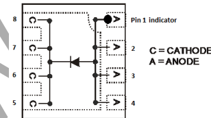
Top View Schematic and Pin Configuration
