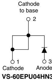
TO-247AC modified
