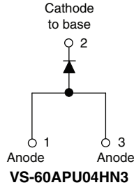
TO-247AC
