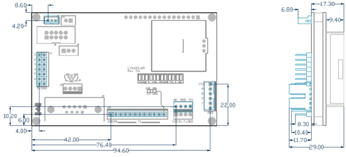
Figure 24: LK204-25-422 Dimensional Drawing
