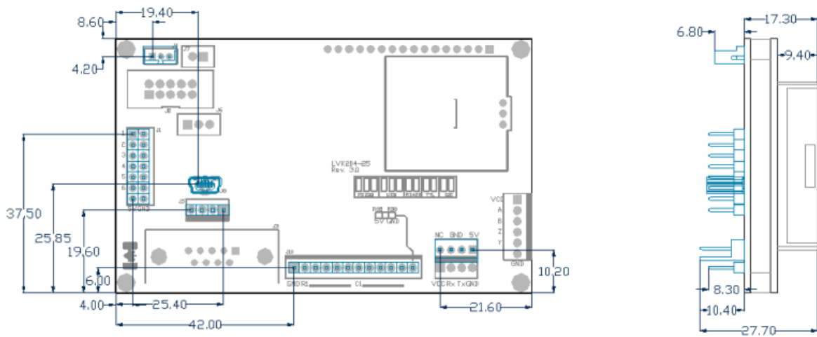
Figure 23: LK204-25-USB Dimensional Drawing
