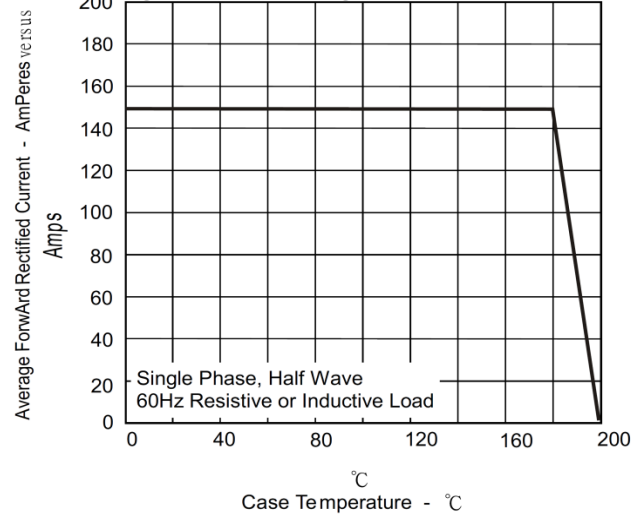
Figur.2-Forward Derating Curve
